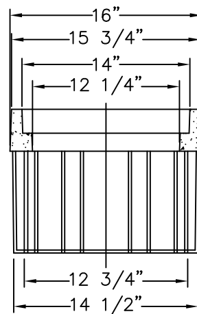
END VIEW
